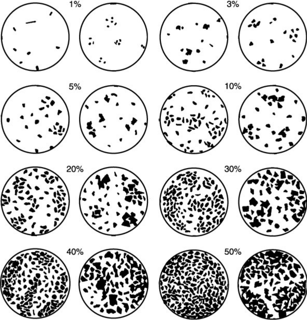
Figure F9. Comparison chart for visual percentage estimation (after Terry and Chilingar, 1955).
